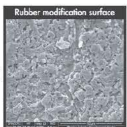
SEM: Rubber surface with graphite modification
